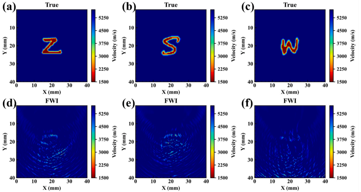
Fig. 7. FWI inversion results of the velocity model with complex geometric defects. (a), (b), and (c) show the true models for the inversions. (d), (e), and (f) show the FWI inversion results corresponding to (a), (b), and (c), respectively.
