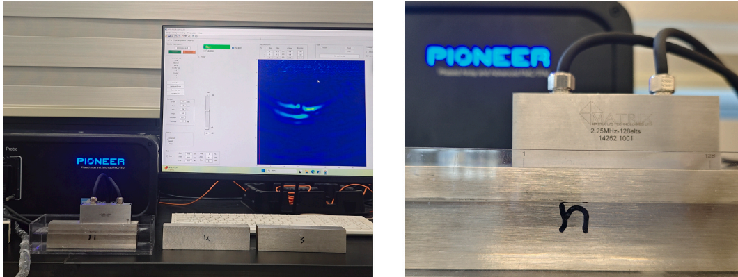
Fig. 10. Experiment setup consisting of a Pioneer Phased Array Acquisition System, a linear phased array, and three specimens.
