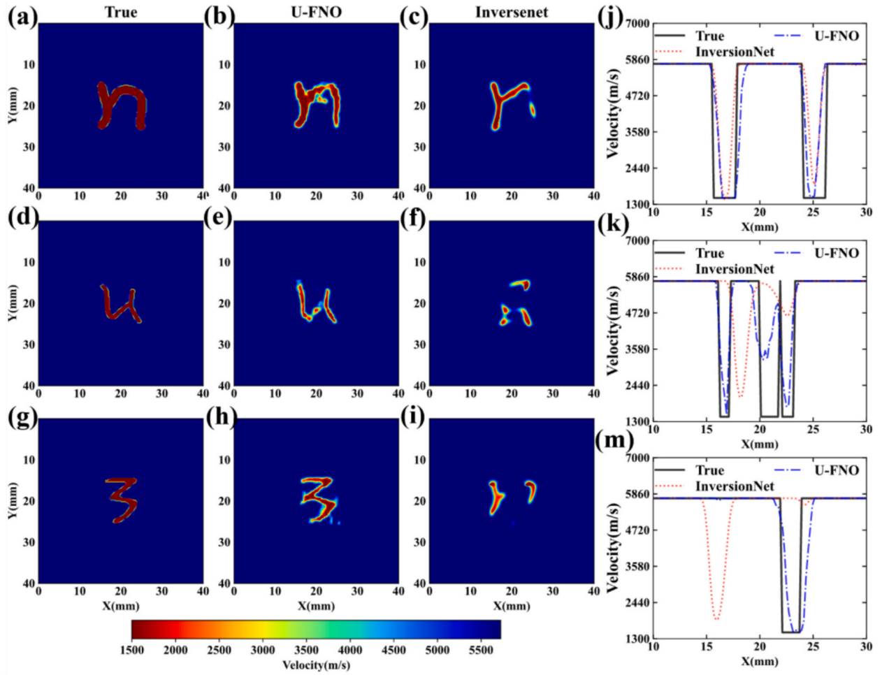
Fig. 11. U-FNO and InversionNet inversion results of the parametric experimental specimens with complex geometric defects in the laboratory. (a), (d), and (g) show the true models for the inversions. (b), (e), and (h) show the U-FNO inversion results corresponding to (a), (d), and (g), respectively. (c), (f), and (i) show the InversionNet inversion results corresponding to (a), (d), and (g), respectively. (j), (k), and (m) show the one-dimensional velocity profiles at y = 21 mm locations extracted from the true model, U-FNO inversion result, and InversionNet inversion result.
