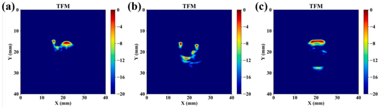
Fig. 12. Conventional TFM image. (a) TFM results corresponding to the model in Fig. 11(a). (b) TFM results corresponding to the model in Fig. 11(d). (c) TFM results corresponding to the model in Fig. 11(g).
