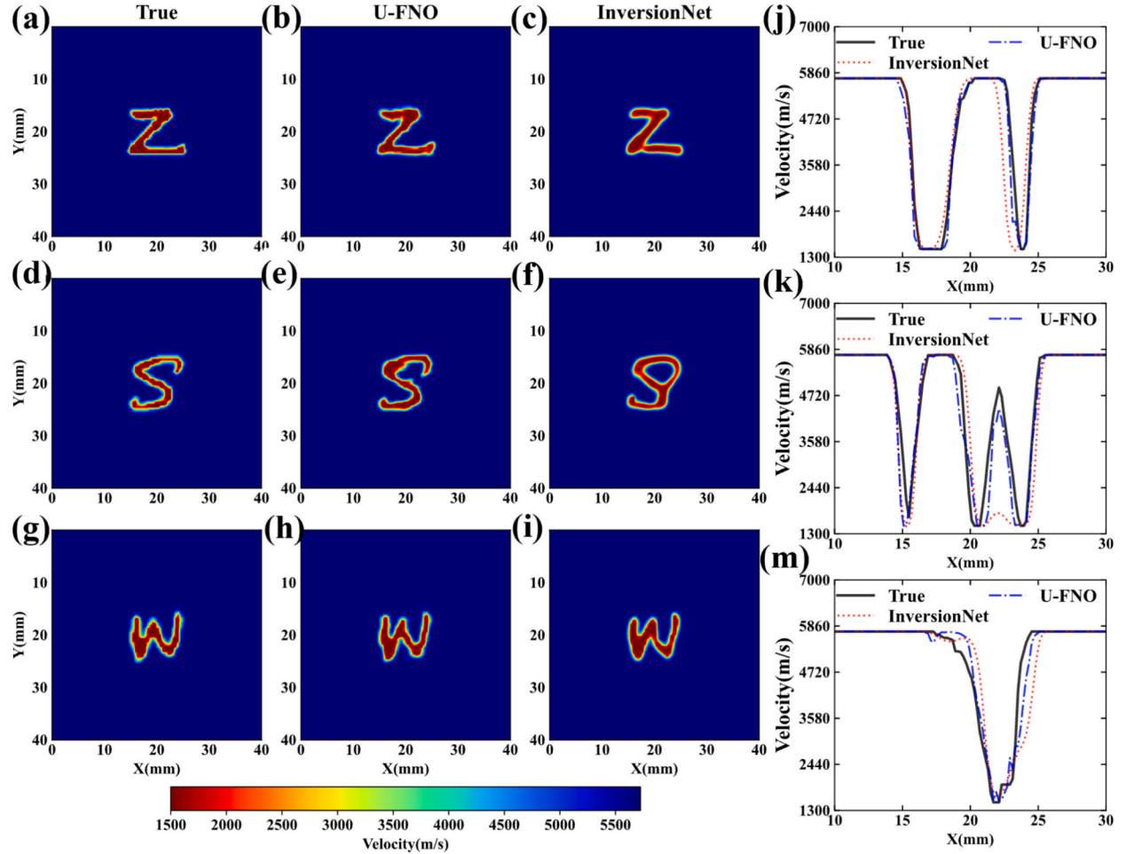
Fig. 5. U-FNO and InversionNet inversion results of the velocity model with complex geometric defects. (a), (d), and (g) show the true models for the inversions. (b), (e), and (h) show the U-FNO inversion results corresponding to (a), (d), and (g), respectively. (c), (f), and (i) show the InversionNet inversion results corresponding to (a), (d), and (g), respectively. (j), (k), and (m) show the one-dimensional velocity profiles at x = 21 mm locations extracted from the true model, U-FNO inversion result, and InversionNet inversion result.
