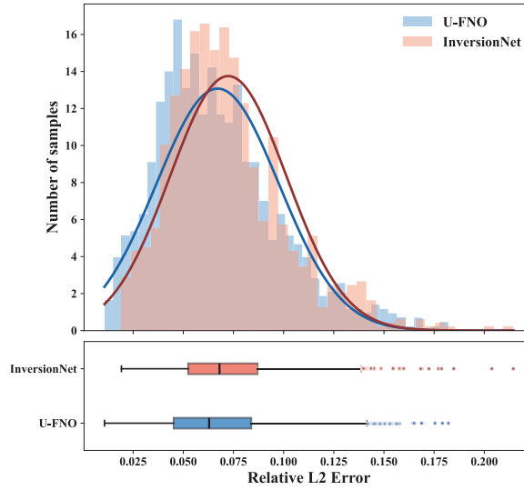
Fig. 6. The distribution of reconstruction errors for 1000 test samples.
