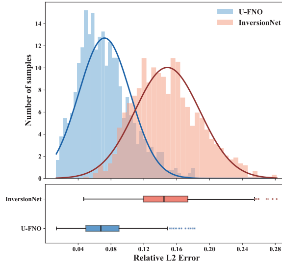
Fig. 9. The distribution of reconstruction errors for 1000 test samples with 6db SNR.
