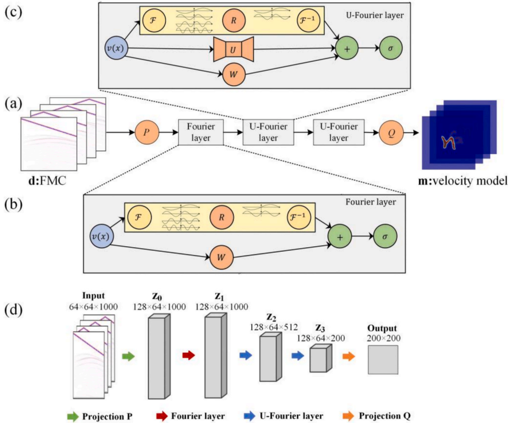
Fig. 3. (a) The U-FNO model architecture. \mathbf{d} is the input, P and Q are fully connected neural networks, and \mathbf{m} is the output. (b) Fourier layer, adapted from [40]. (c) U-Fourier layer, adapted from [53]. (d) Shapes of outputs \mathbf{z}_j , j = 0, 1, 2, 3
