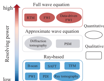
Fig. 1. Acoustic imaging methods based on different theoretical assumptions.
